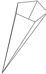
Fig. 9.7. The deformations of the Kähler form that satisfy Eq. (9.94) build the Kähler cone.
